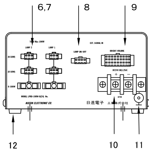
REAR PANEL
